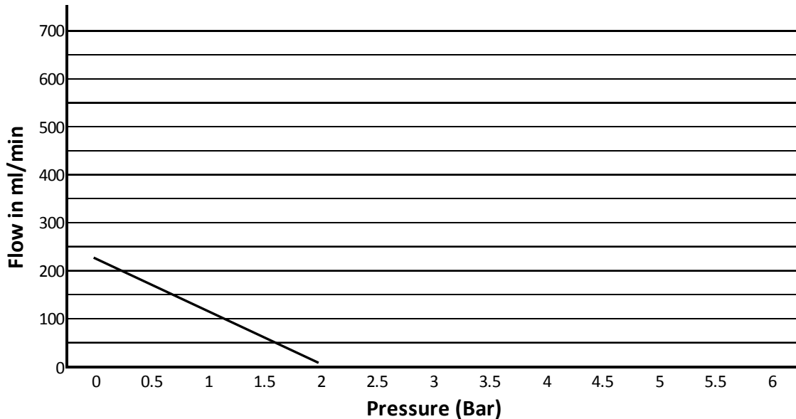
Flow vs. Pressure Curve HP1000.24 at 10 VDC with Water
