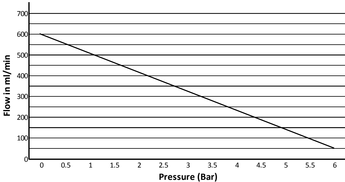
Flow vs. Pressure Curve HP1000.24 at 24 VDC with Water
