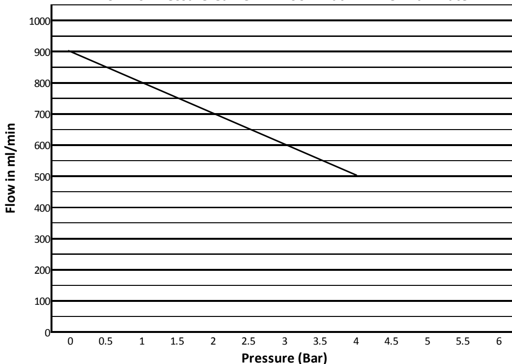
Flow vs. Pressure Curve HP1100.12 at 12 VDC with Water
