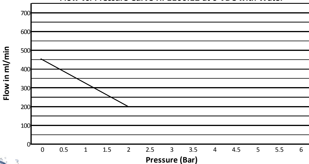
Flow vs. Pressure Curve HP1100.12 at 6 VDC with Water
